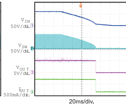
Power Ramp Down V_{IN}=60V , I_{OUT}=0.2A
